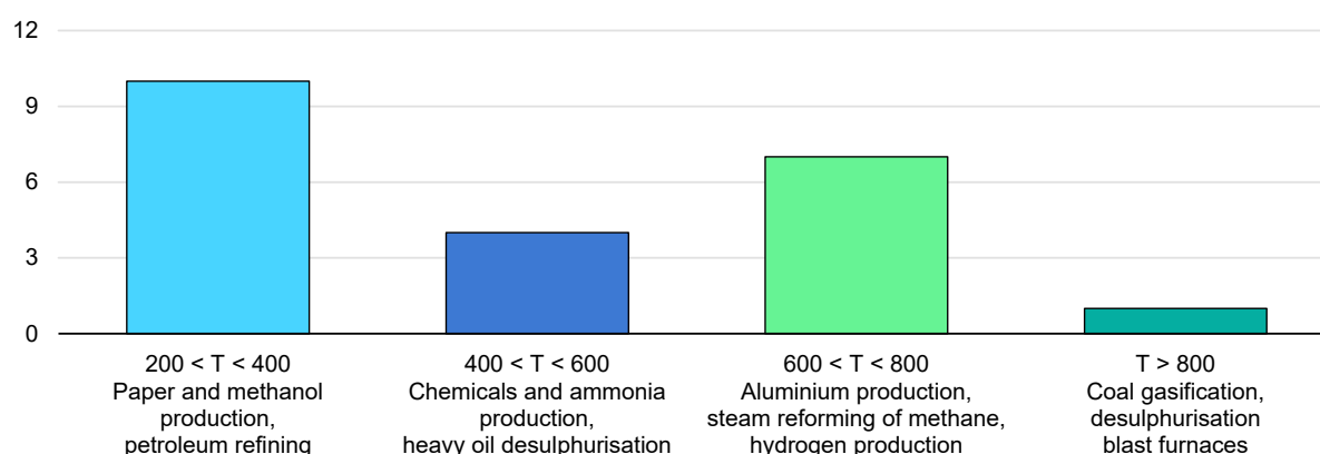
Number of leading SMRs projects globally by temperature range and targeted use
