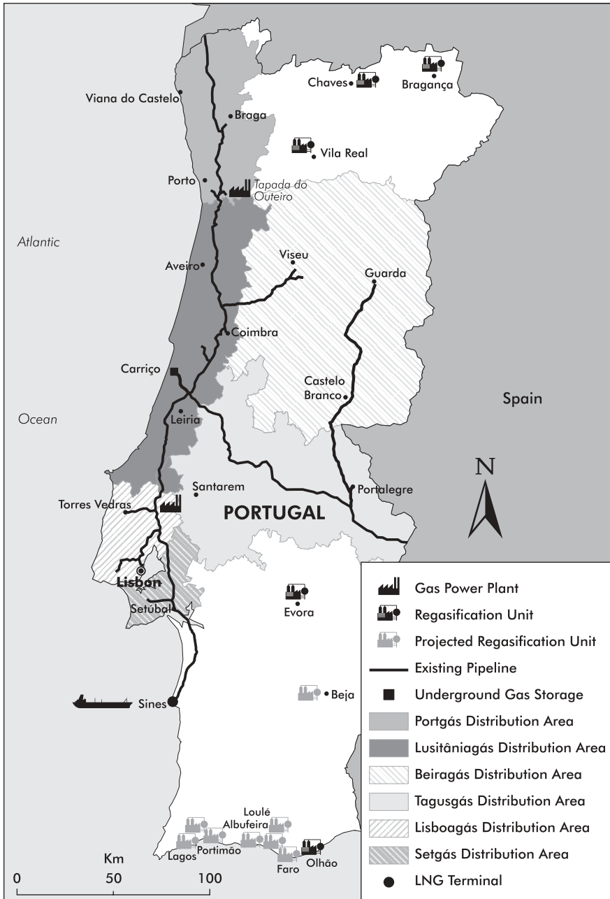
Figure 16 Natural Gas Infrastructure
