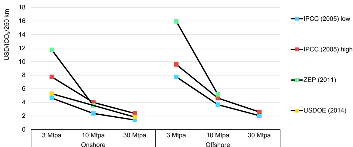
Figure 3.6 Indicative unit CO 2 pipeline transport costs
