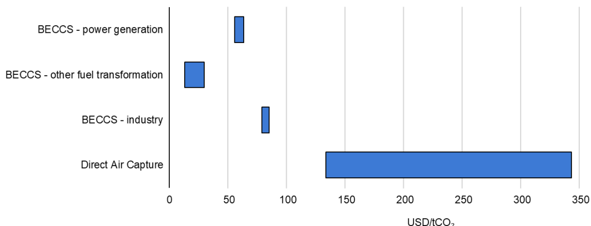
Figure 2.18 Current cost of CO 2 capture for carbon removal technologies by sector
