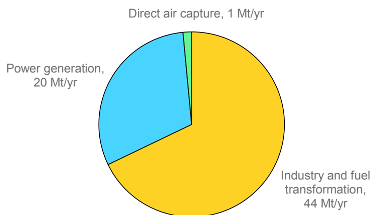
Figure 5.1 World CO 2 capture capacity average annual additions to 2030 by sector in the Sustainable Development Scenario
