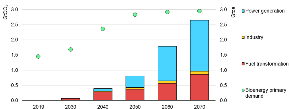
Figure 2.20 Global CO 2 capture from BECCS by sector (left) and bioenergy primary demand (right) in the Sustainable Development Scenario
