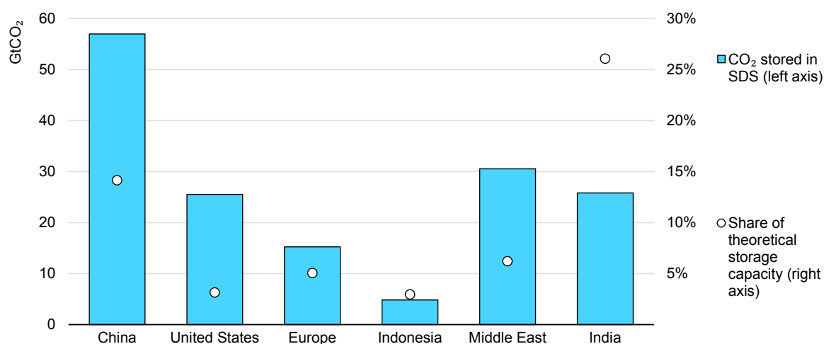
Figure 3.9 Theoretical CO 2 storage capacity and cumulative CO 2 storage in the Sustainable Development Scenario by region
