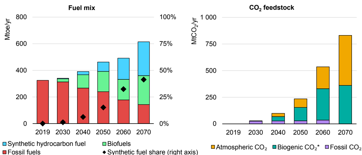
Figure 2.13 Global energy demand in aviation and CO 2 use as feedstock for synthetic kerosene in the Sustainable Development Scenario
