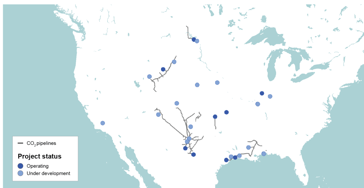
Figure 3.5 Existing CO 2 pipeline infrastructure and CCUS projects in the United States
