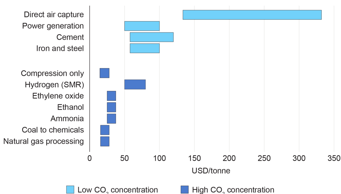
Figure 3.4 Levelised cost of CO 2 capture by sector and initial CO 2 concentration, 2019
