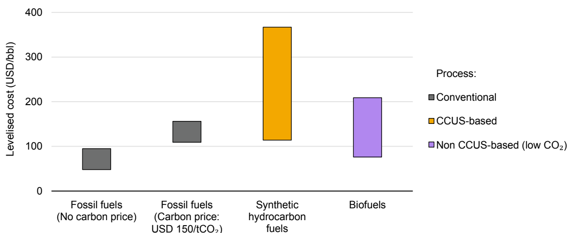
Figure 2.12 Simplified levelised cost of low-carbon fuels for long distance transport
