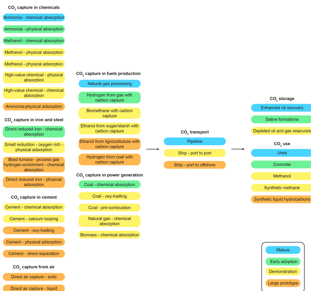
Figure 3.1 TRL of select technologies along the CCUS value chain
