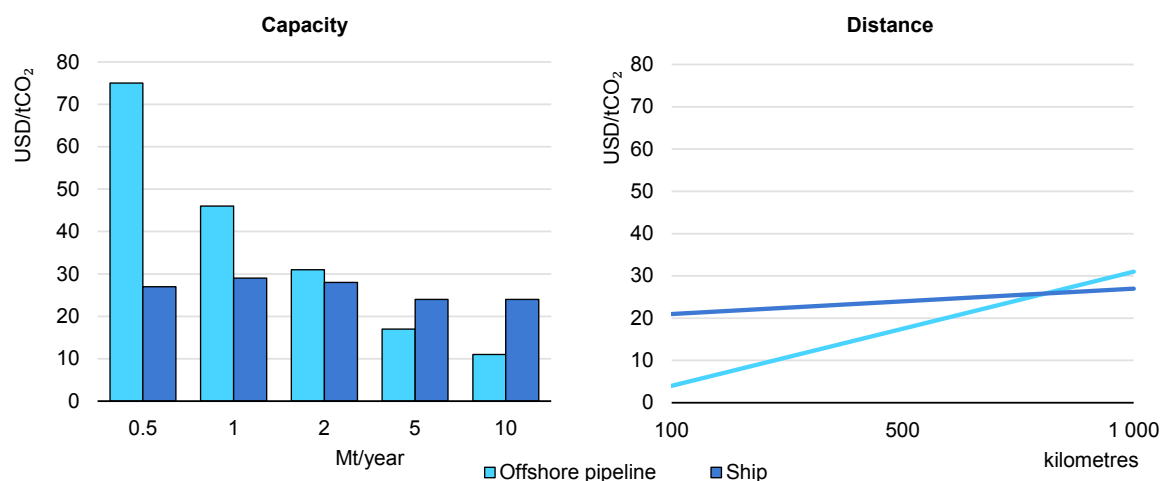
Figure 3.7 Shipping and offshore pipeline transportation costs
