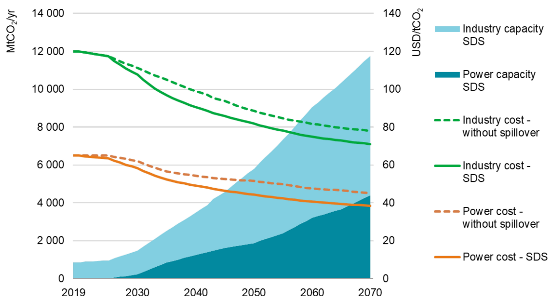
Figure 3.11 Cumulative capacity (left) and capture cost learning curve (right) for CO 2 chemical absorption in coal-fired power generation and small industrial furnaces in the Sustainable Development Scenario
