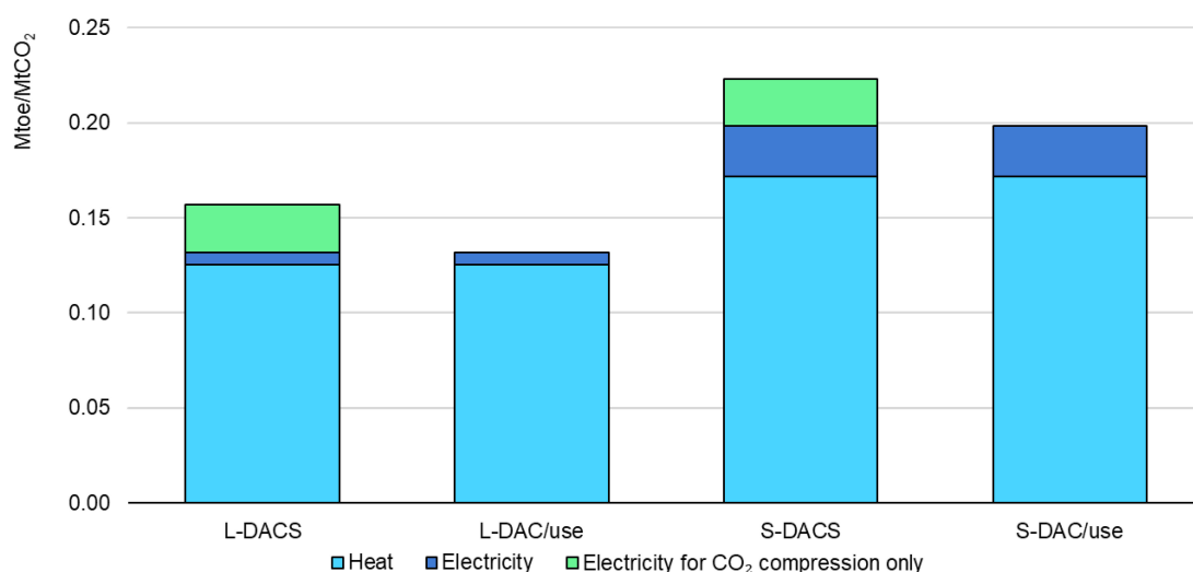
Figure 2.17 Specific energy consumption for CO 2 capture using current DAC technologies
