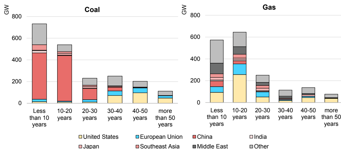
Figure 2.7 Age structure of existing coal and gas power capacity by region
