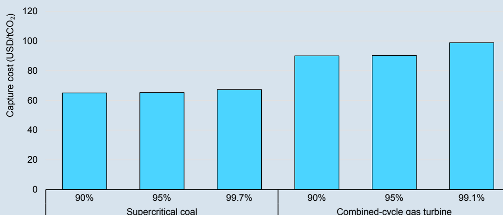
Indicative CO 2 capture costs for coal- and gas-fired power plants by capture rate
