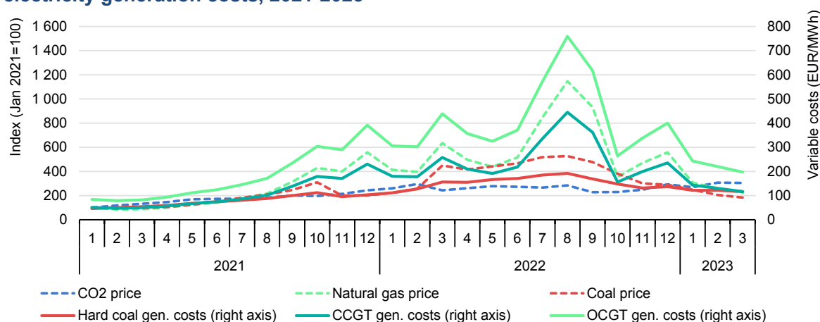
EU CO 2 emissions allowances, natural gas prices, coal price index, and variable electricity generation costs, 2021-2023
