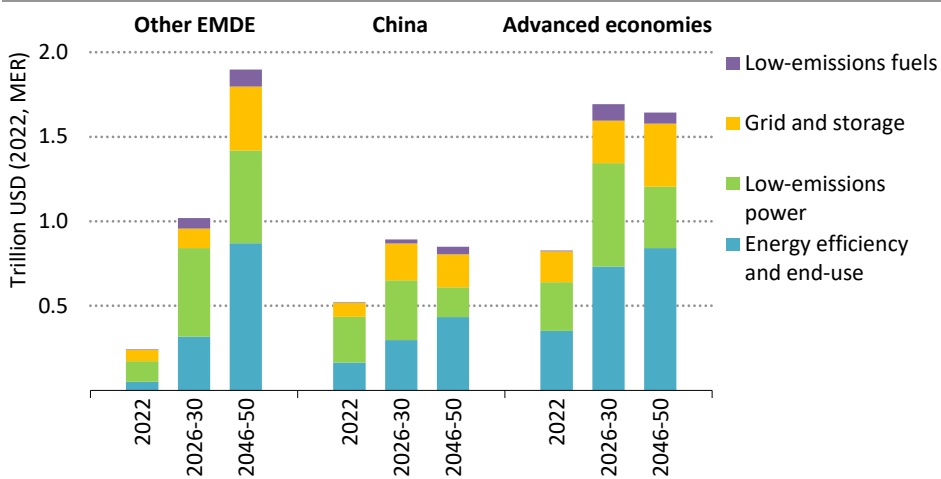
Figure 4.13 ▶ Clean energy investment needs by region/country in the NZE Scenario, 2022-2050
