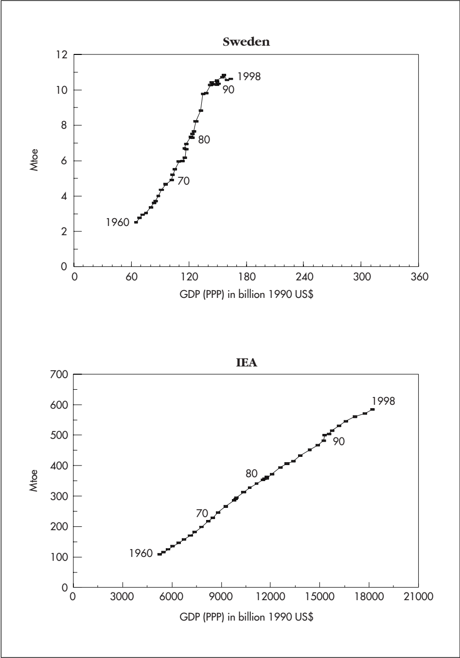
Figure 13 Electricity Consumption vs GDP in Purchasing Power Parities, 1960-1998
