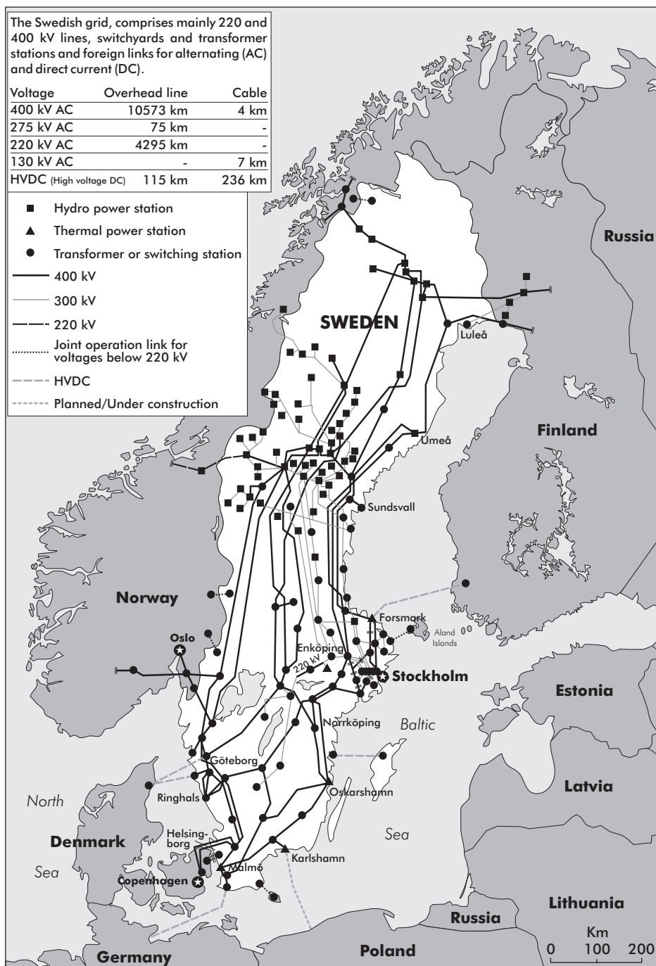
Figure 18 Swedish National Electricity Grid
